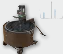
Automix 1801 1500 W; 50 rpm 65 l; up to 50 kg mixture
